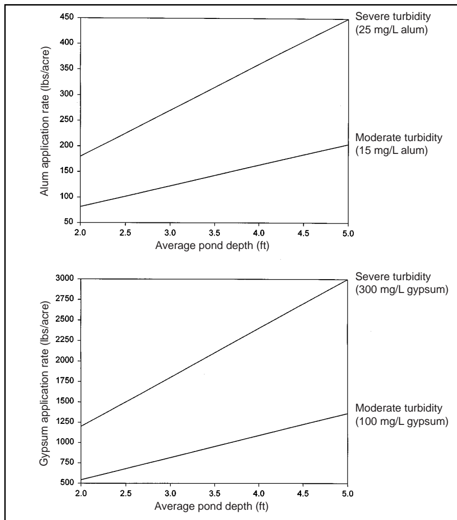
Figure 4. Guidelines for alum and gypsum application rates are a function of pond depth and the severity of the turbidity problem.
