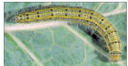
Figure 15. Ascia monuste .
